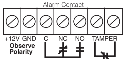
Contacts shown energized in the non-alarm state
